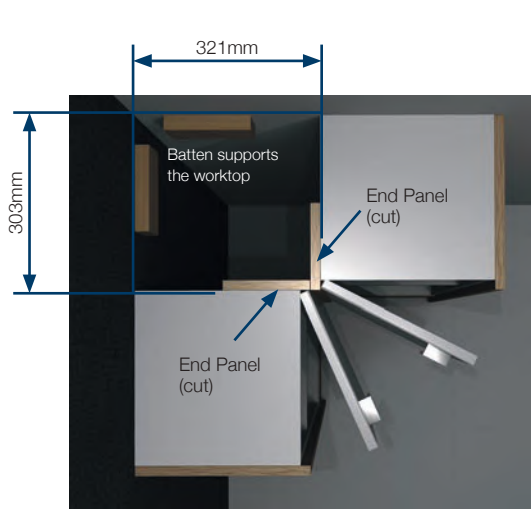
Layout 1: Suitable for doors only. (Using end panels in corner)
