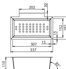
Stainless Steel Colander Ref. COL106 £70
