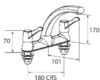
Mercia QT lever deck sink mixer
