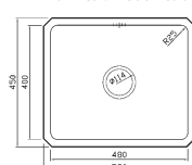
Salsa Single bowl Ref. SA48 £371
