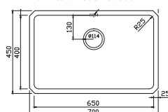
Salsa Single bowl Ref. SA65 £463
