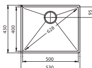
Stereo Single bowl Ref. STE50 £400
