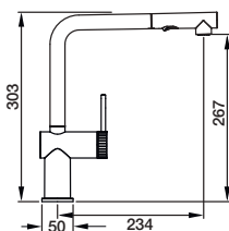
Fraction single lever monobloc with swivel spout and pull-out spray
