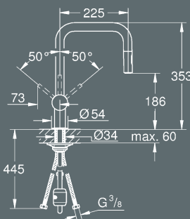
Minta single lever monobloc with extractable trigger spray/mousseur
