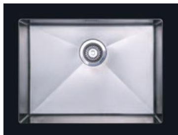
Jazz Single bowl Ref. JA013 £314 Overall size: 590/440 mm Bowl size: 550/400/190 mm Min cabinet size: 600 mm
