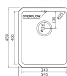
Salsa Single bowl Ref. SA34 £305
