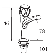
Mercia Modern Sink Pillars
