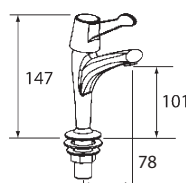
Mercia QT Lever Sink Pillars
