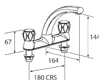
Mercia Modern deck sink mixer with twin controls
