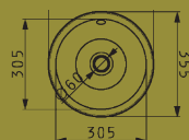
Arco Mini Single bowl Ref. 25201 £192 Overall size: Ø355 mm Bowl size: Ø305/170 mm Cutout size: Ø335 mm Minimum cab size: 350 mm Waste included: 60 mm BSW
