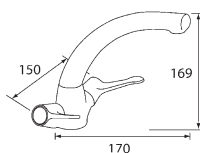
Mercia QT Lever Sink Mixer
