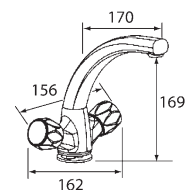
Mercia Modern Sink Mixer
