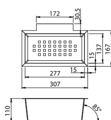
Stainless Steel Colander Ref. COL107 £70
