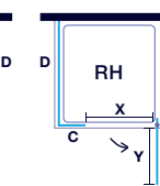
Pivot Door & Inline Panel with Side Panel
