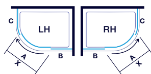
1 Door Offset Quadrant
