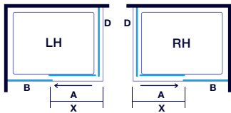
Sliding Door with side Panel
