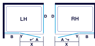
Hinge and Inline Door with Side Panel
