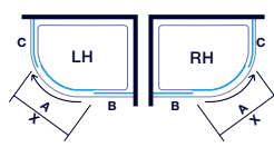
1 Door Offset Quadrant
