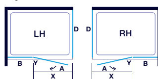
Hinge and Inline Door with Side Panel
