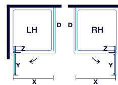
Pivot Door with Side Panel
