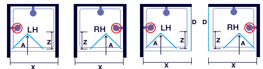
Bifold Door in Recess
