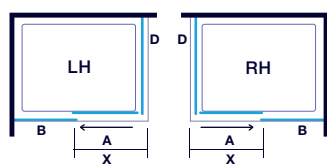
Sliding Door with Side Panel
