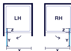
Pivot Door in Recess
